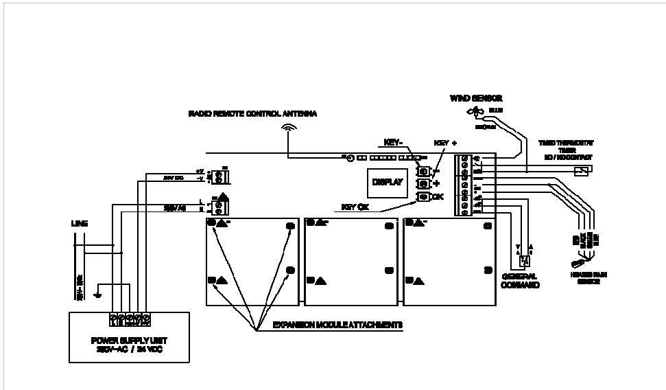
Fig. 7.1 Main Board
