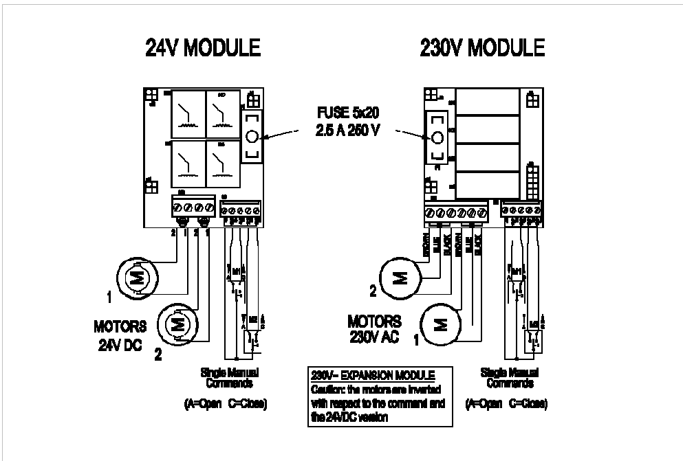
Fig. 7.2 Expansion Modules
